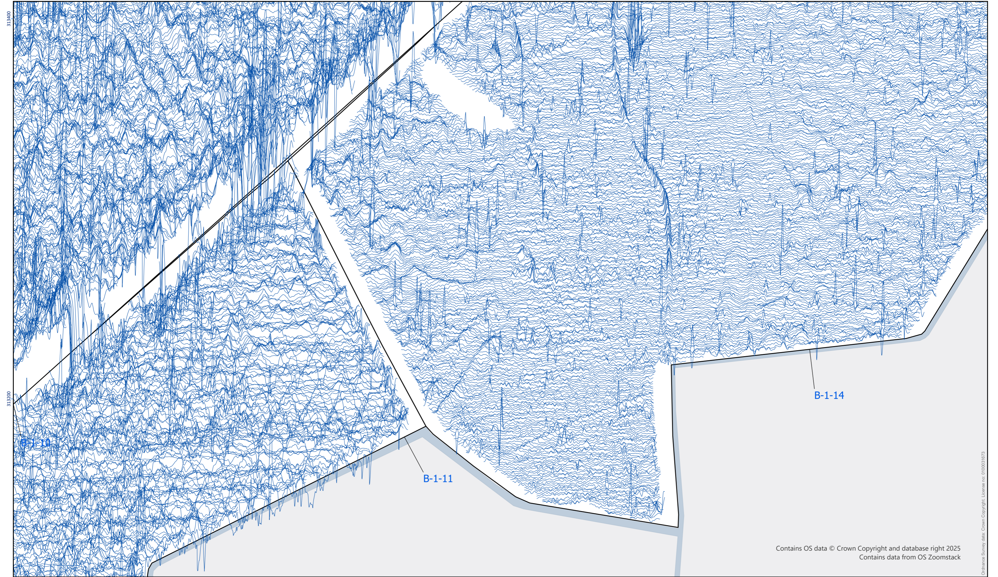
Minimally Processed Gradiometer Data – XY Trace
